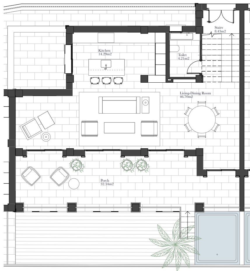
Ground Floor 1:100
