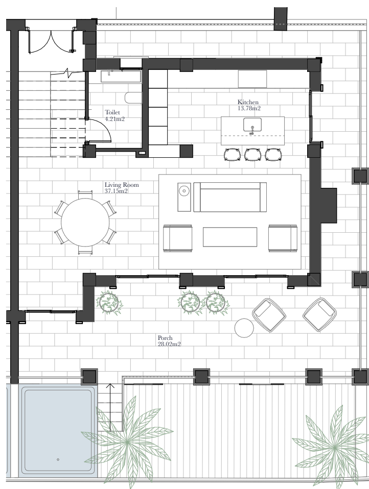
Ground Floor 1:100
